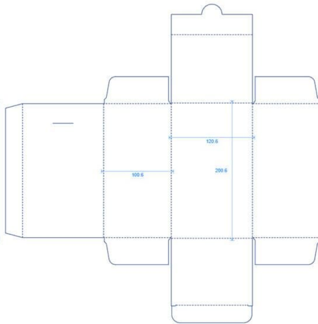
Exterior Dimensions
